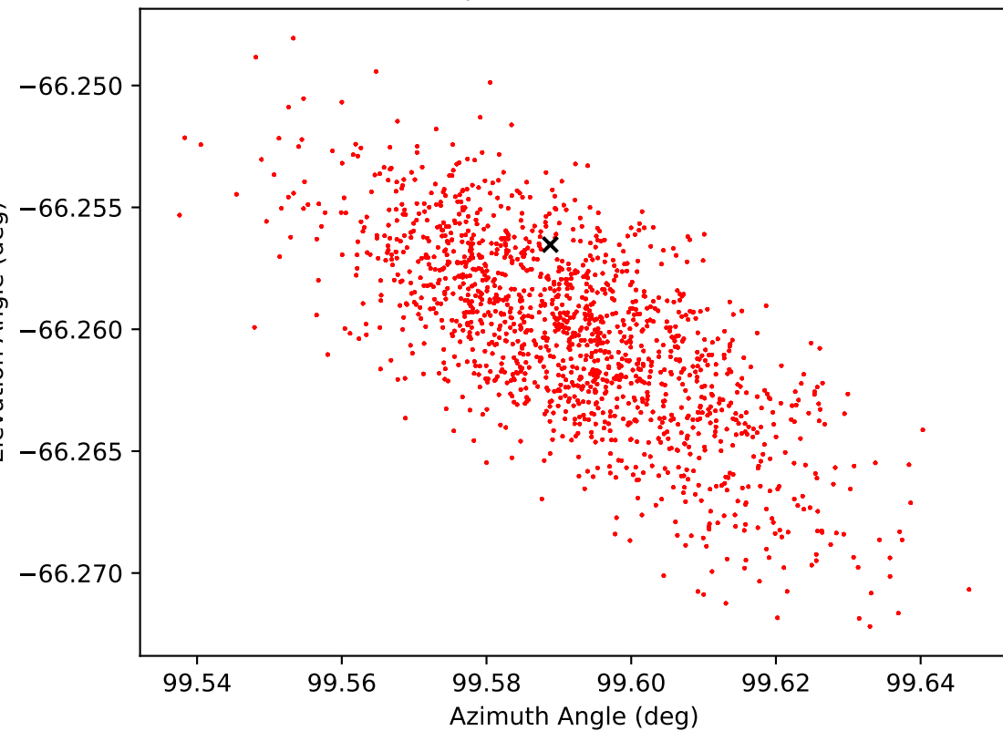
Timestep 50.8014 Hours (Post)
